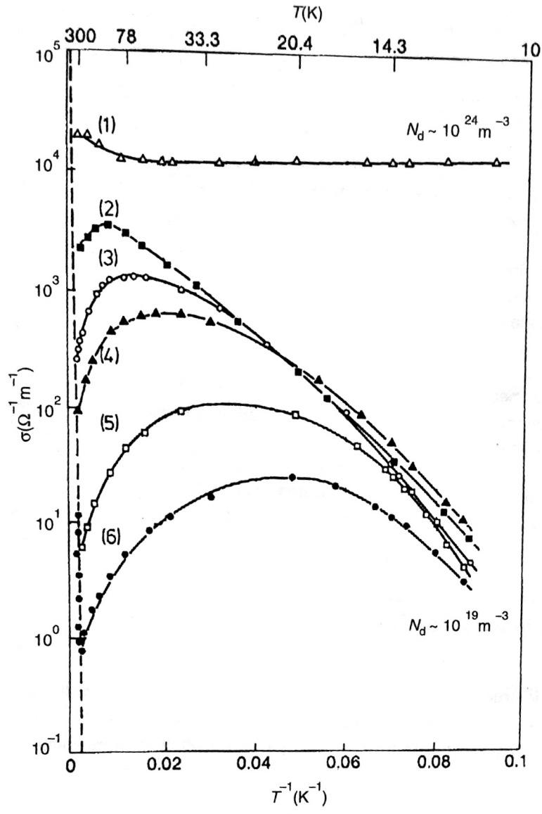
Temperature dependence of the electronic conductivity of n-type Ge.
