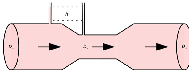
Figure 1. Venture tube.
