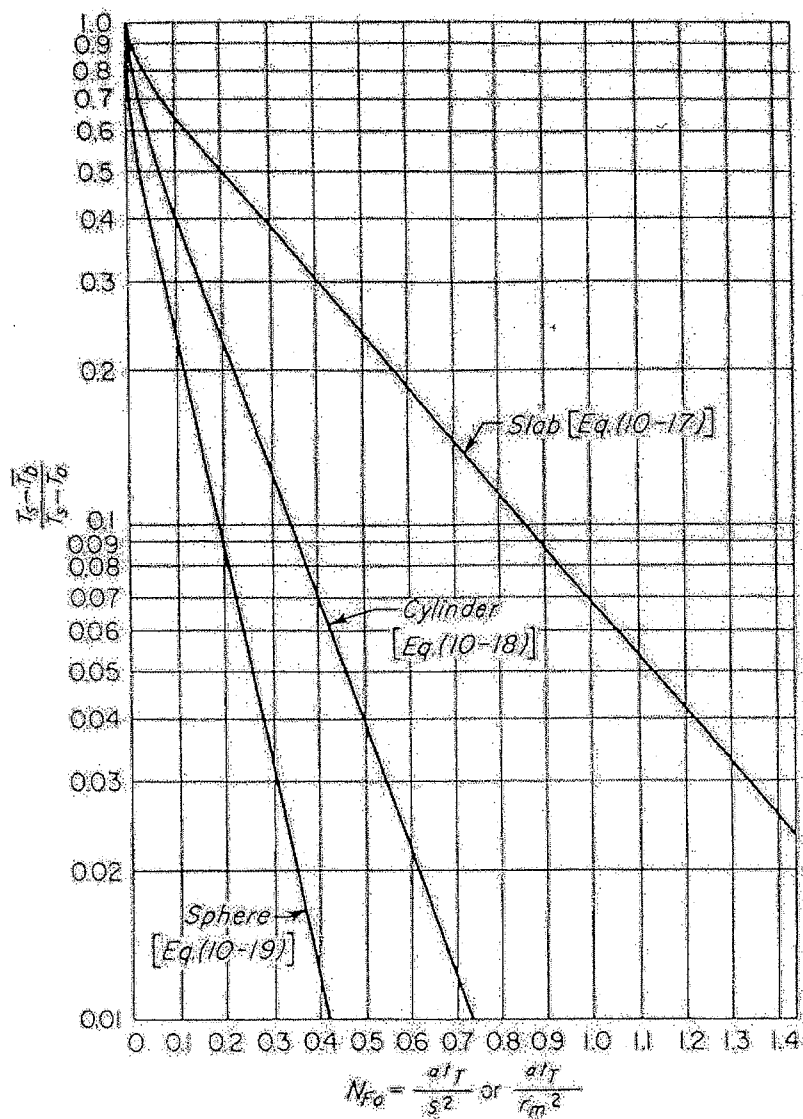
Figure 10-6 Average temperatures during unsteady-state heating or cooling of a large slab, an infinitely long cylinder, or a sphere.
