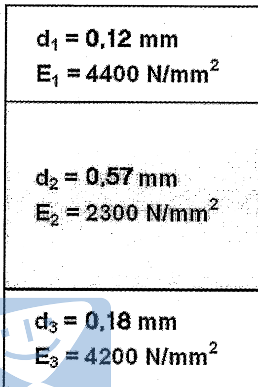
Figure 1. Structure of a 3-layer board (question 5)
